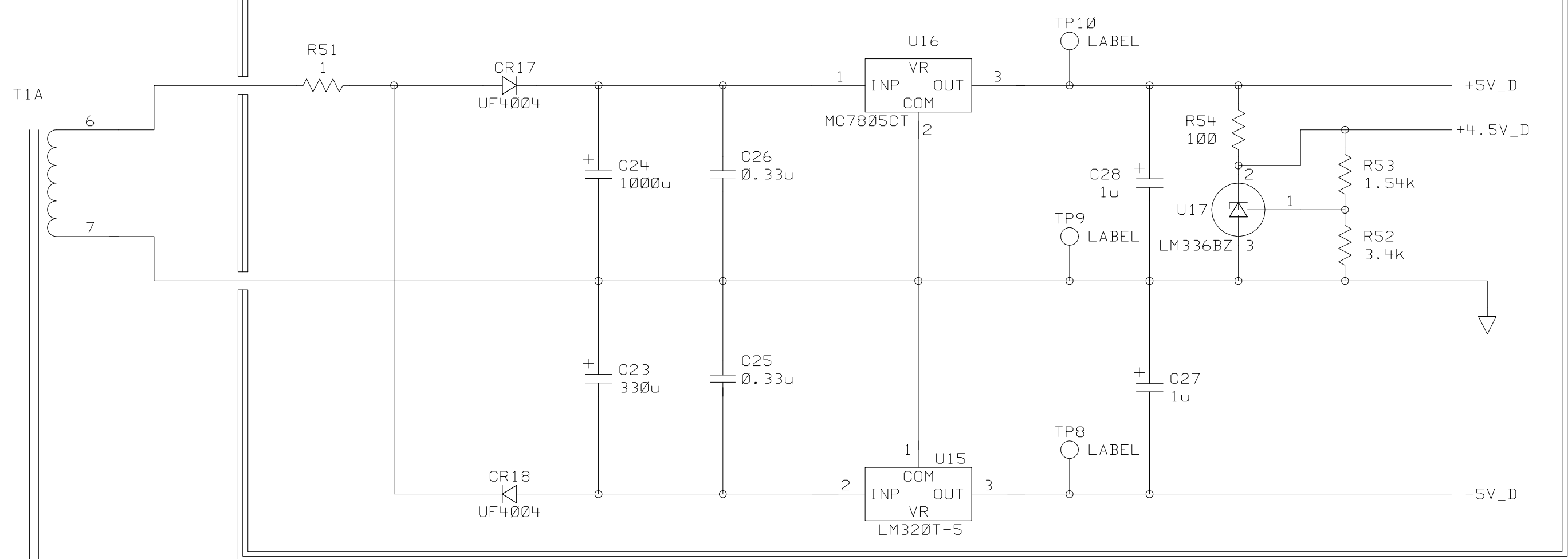
Ⓐ Display Board Bias & Reference Circuit
