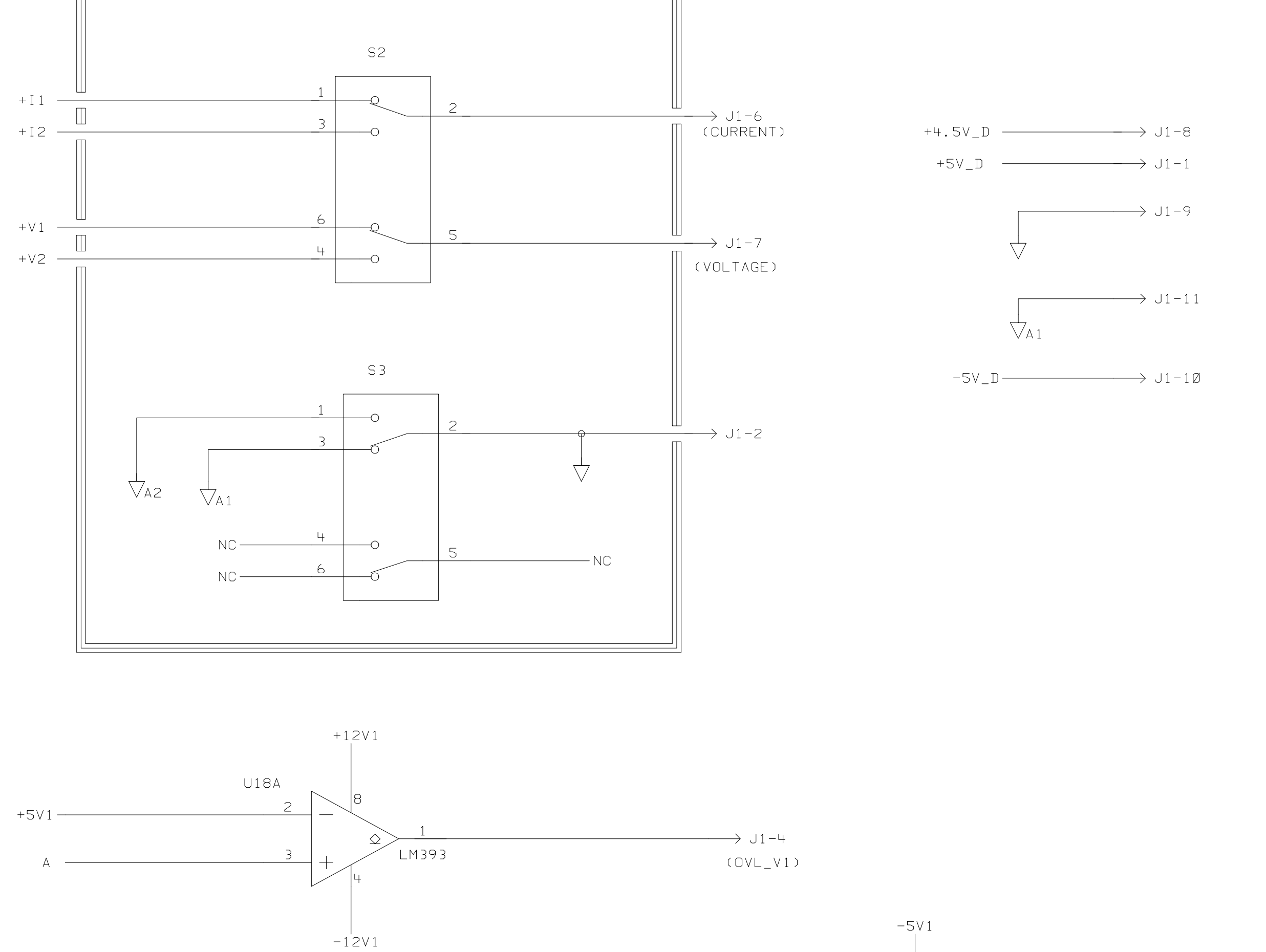
Ⓒ Meter Select Circuit
