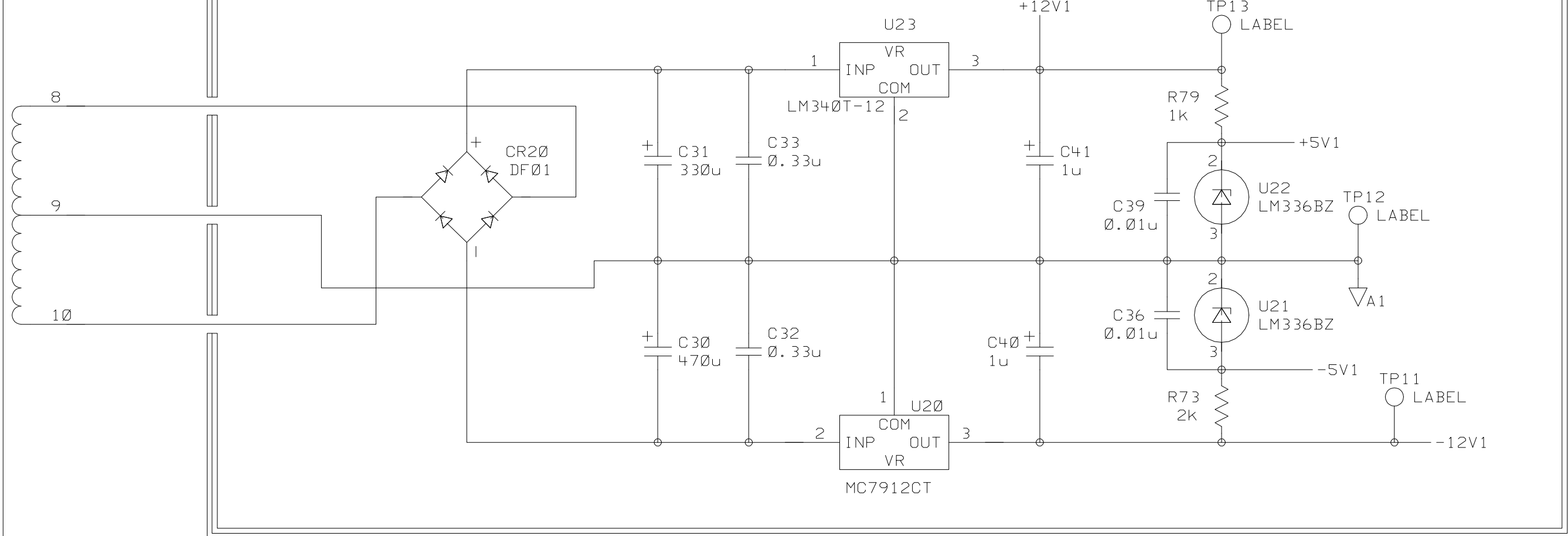
Ⓑ V1 Output Bias & Reference Circuit
