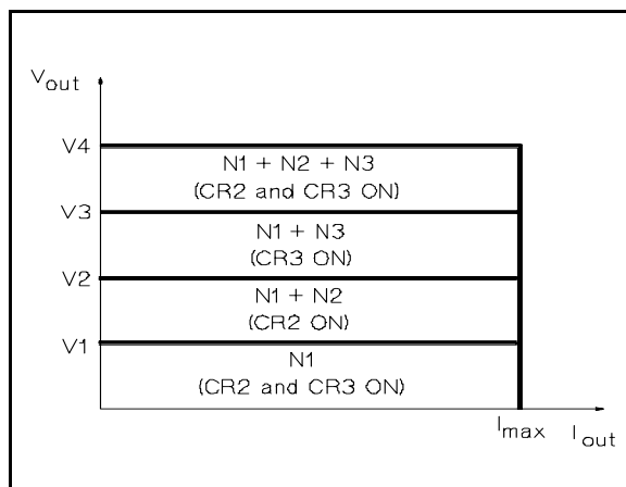
Figure A-2. Output Power Plot
