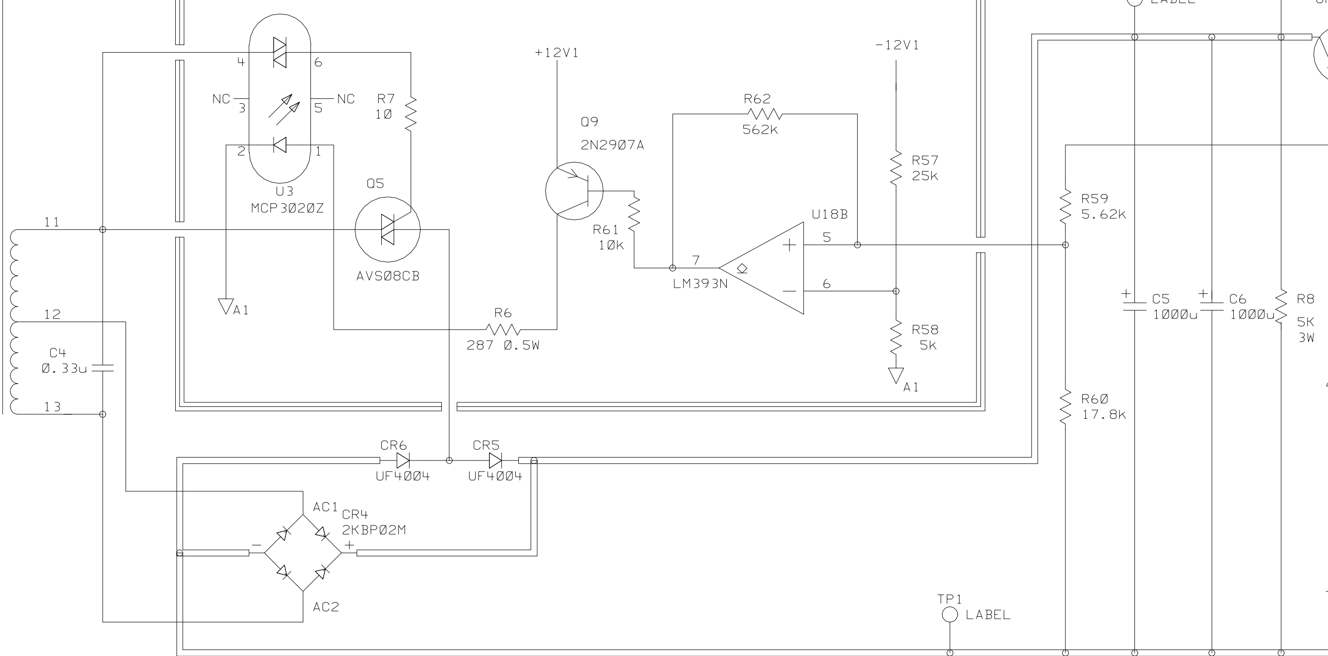
Ⓓ V1 Output TRIAC Control Circuit
